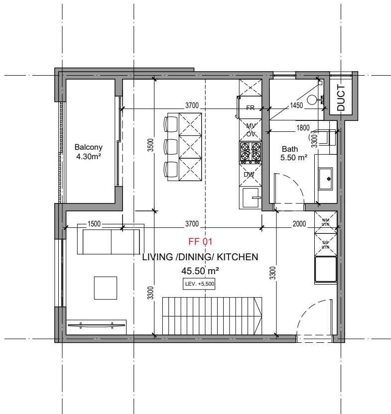
FIRST FLOOR [ APARTMENT 1 ]
